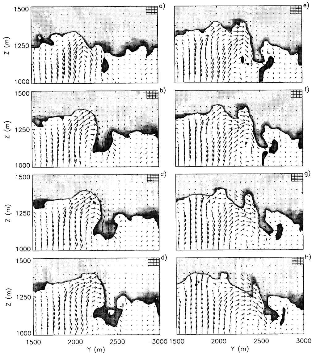
FIG. 8. Temporal and spatial evolution of the inversion interface in a limited domain. Temperature contours as in Fig. 7 along with flow vectors ( v , w ). Only every third grid point in z and every second grid point in y is shown for clarity. Panels (b)–(h) are 107, 134, 161, 228, 255, 295, and 335 s, respectively, later than (a).
