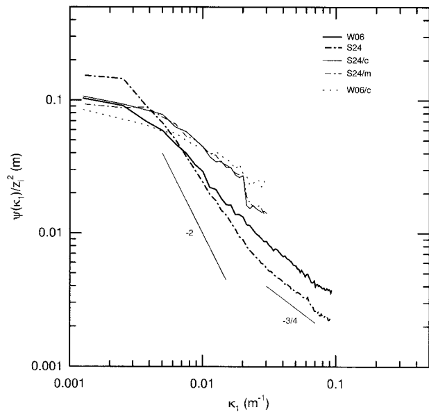
FIG. 18. One-dimensional spectra of z_i fluctuations normalized by z_i^2 for different simulations. In mixing-box experiments, Perera et al. (1994) found a \kappa_1^{-2} spectral slope in the regime where intermittent wave breaking was observed.
